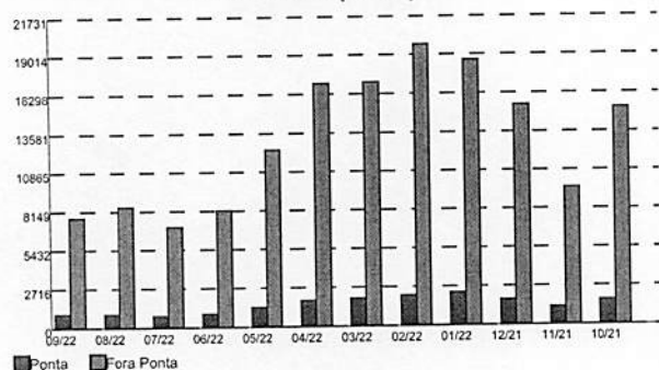
Consumo (kWh)
